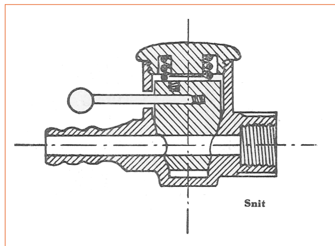
Snit i gashane. HFB 6, 1936.
